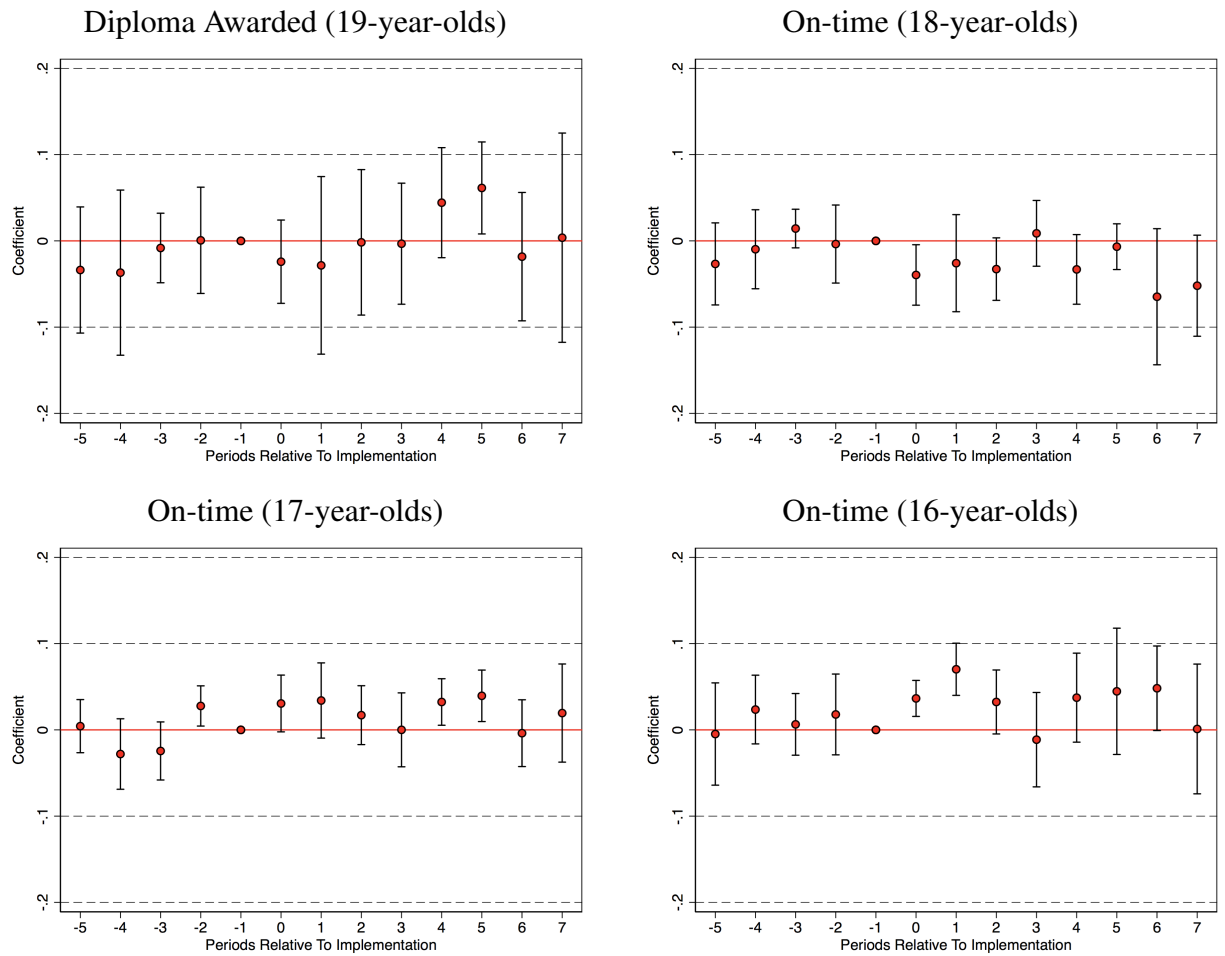
Figure 2: Event Study
