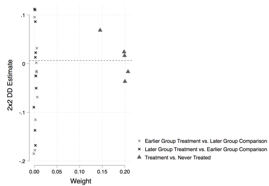
Figure 3: Bacon Decomposition
